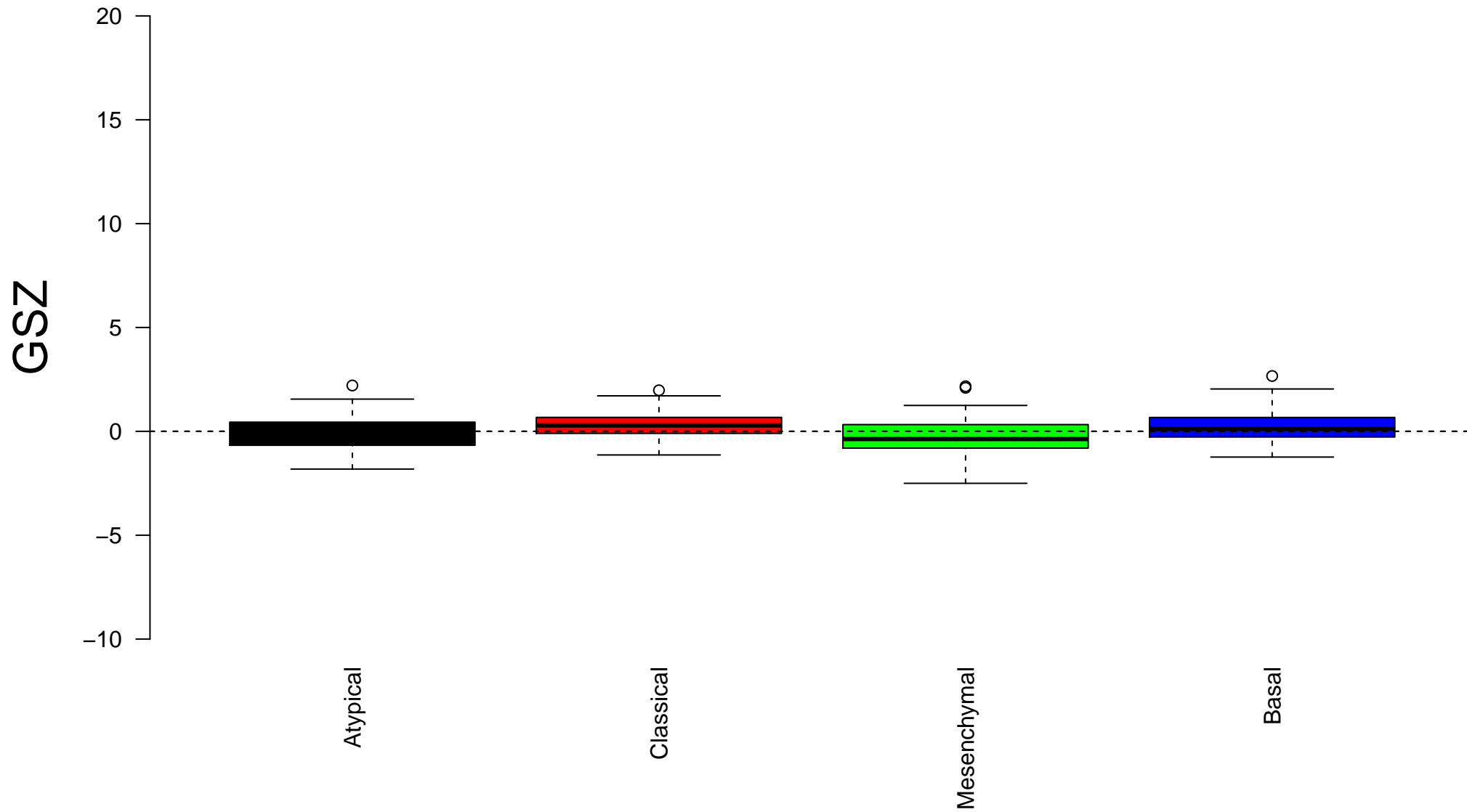
willscher_GBM_Verhaak-CL_expression_K_down
